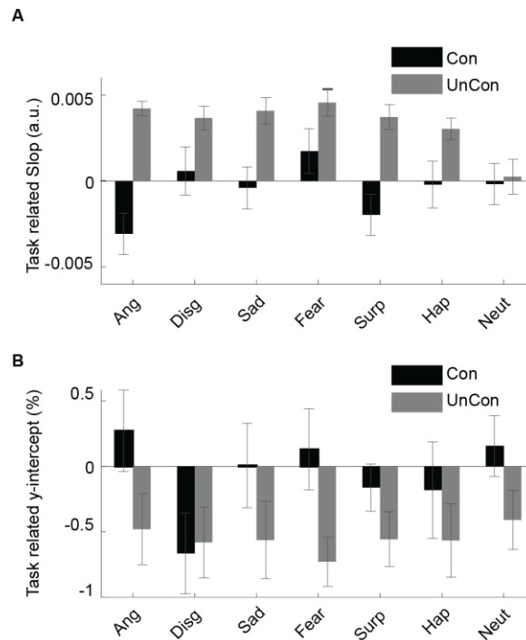
Figure 6. Task related Model parameters over subjects. Tasl related parameters, upper plot slope of line and lower plot y- intercept.
